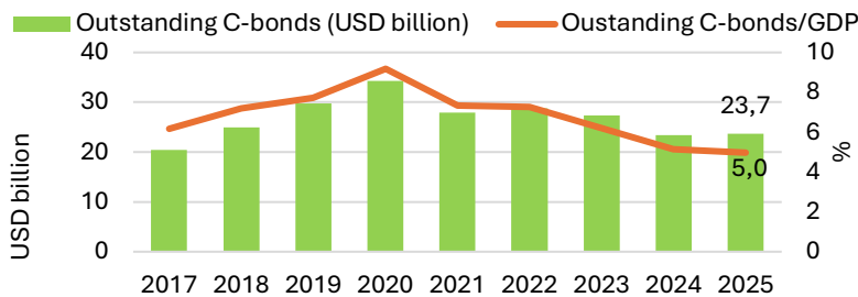
Figure 35: Outstanding C-bonds
